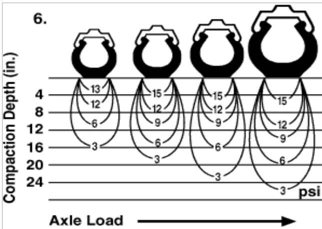
Figure 2.8.a – Soil Compaction and Depth Exhibit.
